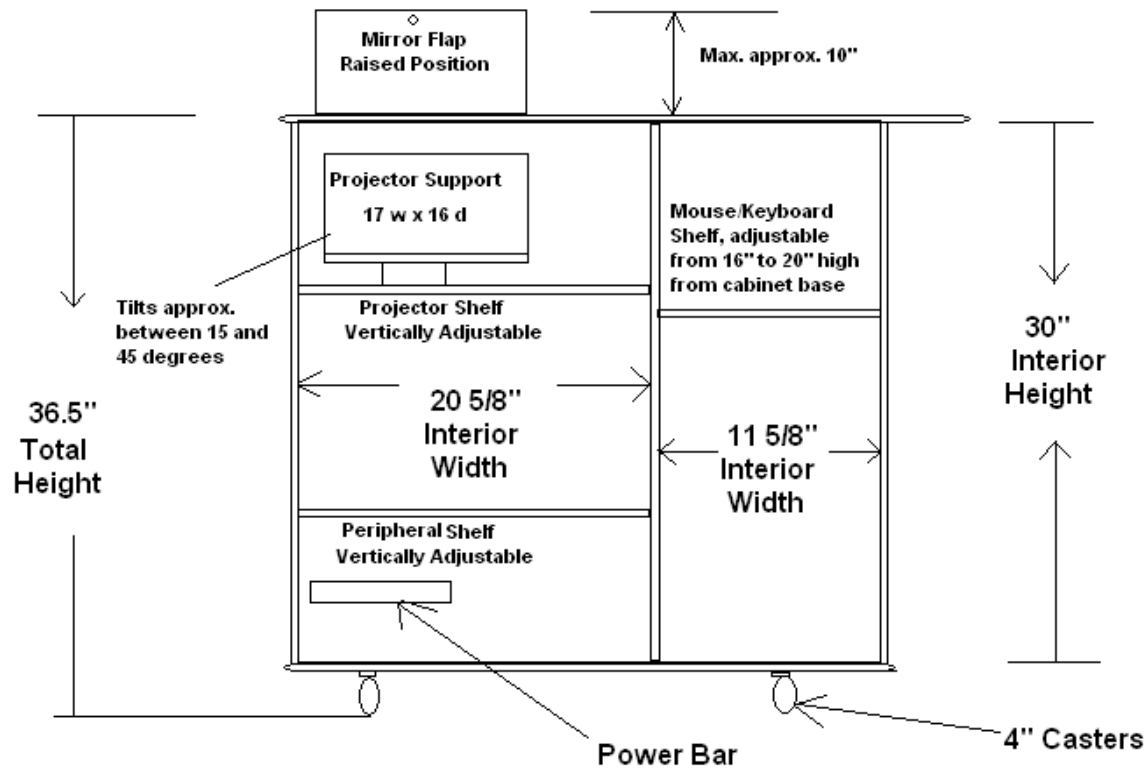
Presenter Side View Doors not Shown
